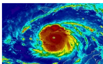
Myanmar Cyclone
