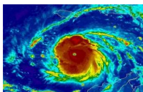
Harricane Gustav
