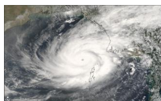
Myanmar Cyclone
