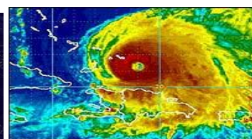
Hurrican Ike
