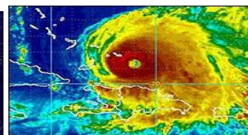
Hurricane Ike
