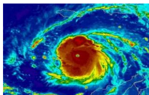
Hurricane Gustav
