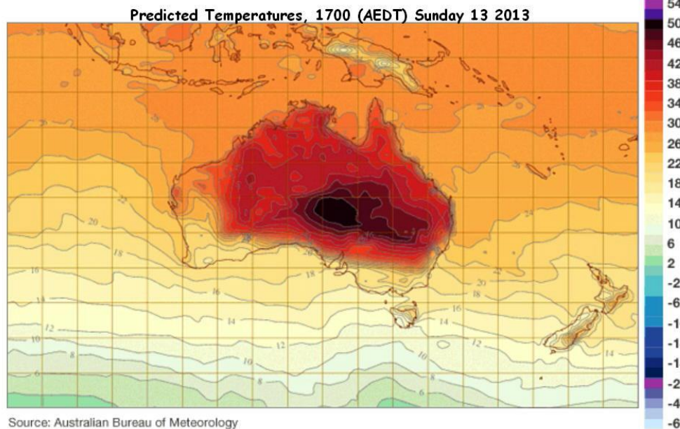
Predicted temperatures, 1700 (AEDT) Sunday 13 Jan
