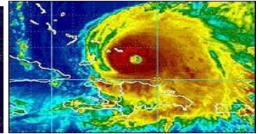
Hurricane Ike
