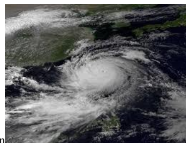
Typhoon Wipha
