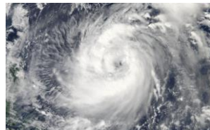
Typhoon Fitow
