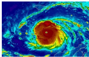
Hurricane Gustav
