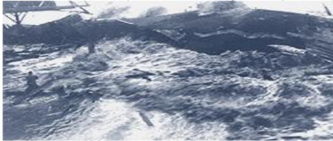
From the NOAA Photo Library, public domain Tsunami inundating Hilo, Hawaii. Note man on pier.
