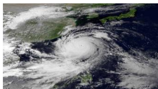
Typhoon Usagi
