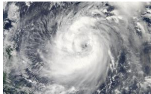
Typhoon Fitow
