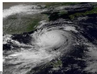
Typhoon Wipha
