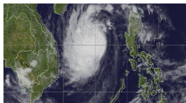
Typhoon Nari
