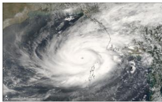
Myanmar Cyclone
